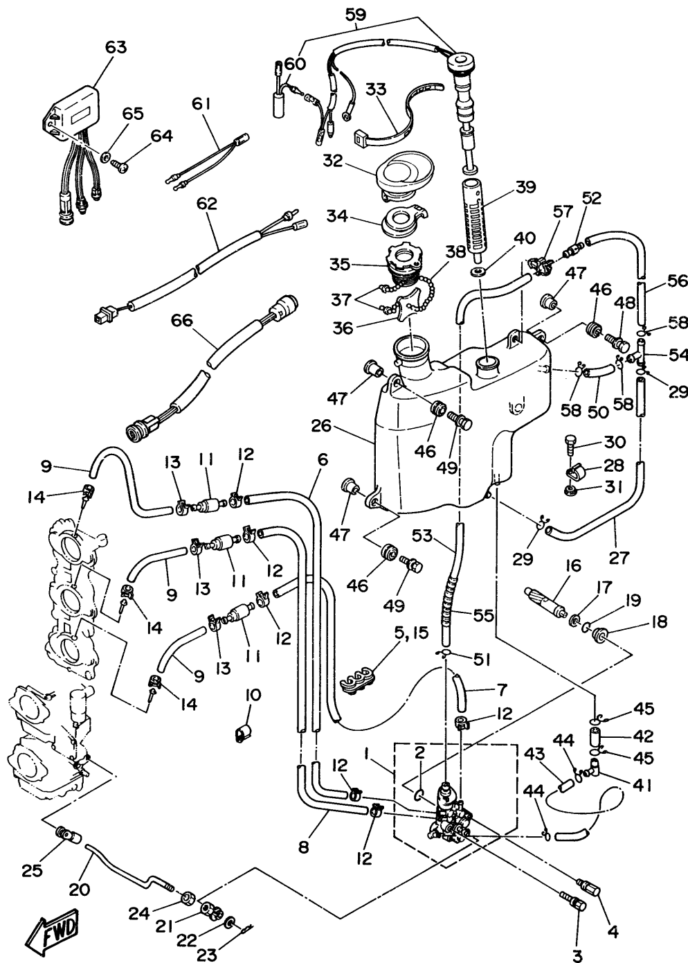
Fig. 5 OIL PUMP
