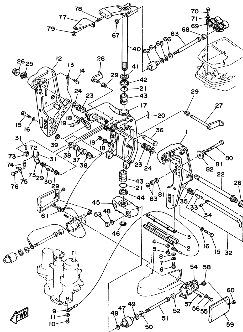
Fig. 11 BRACKET 2 (LONG TRANSM)
