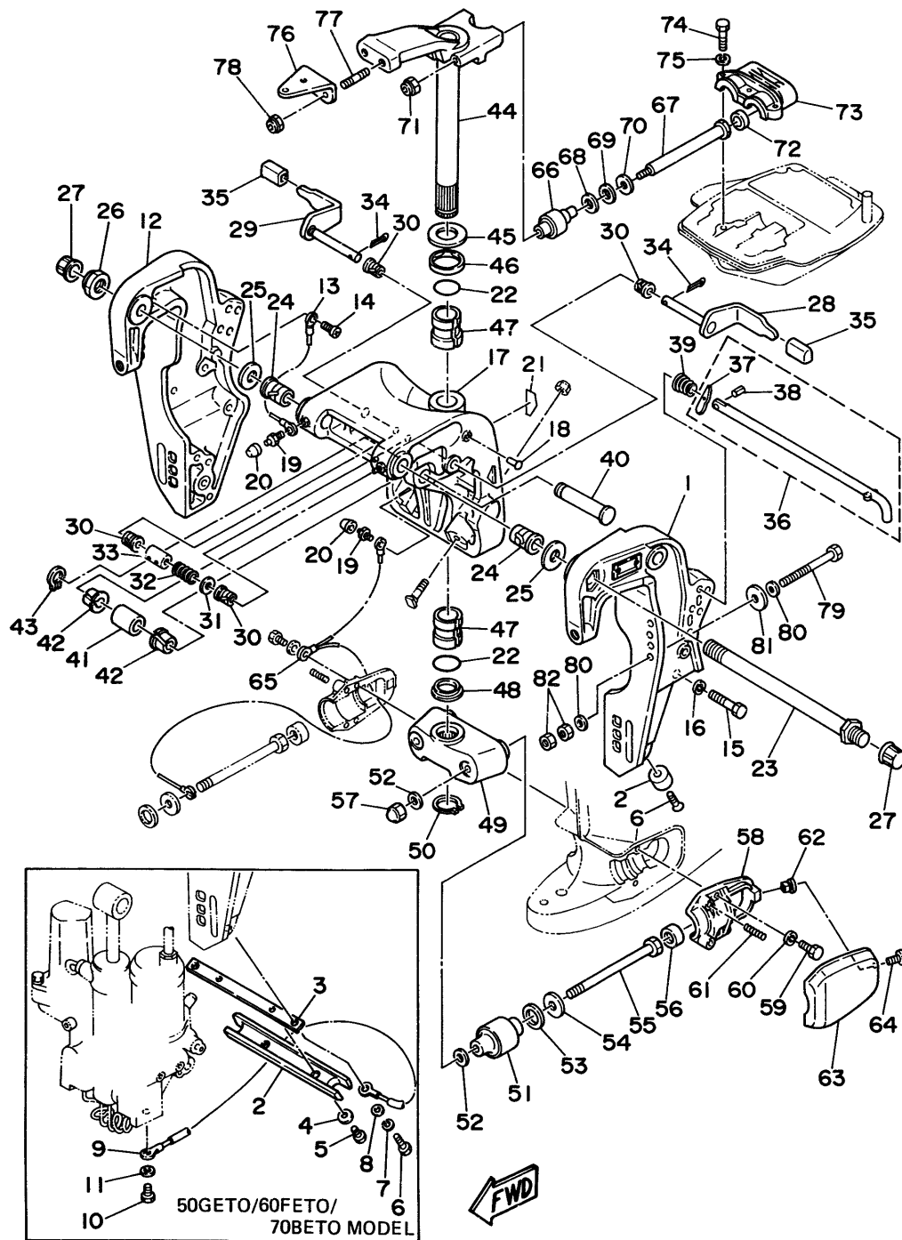
Fig. 10 BRACKET 1 (SHORT TRANSOM)
