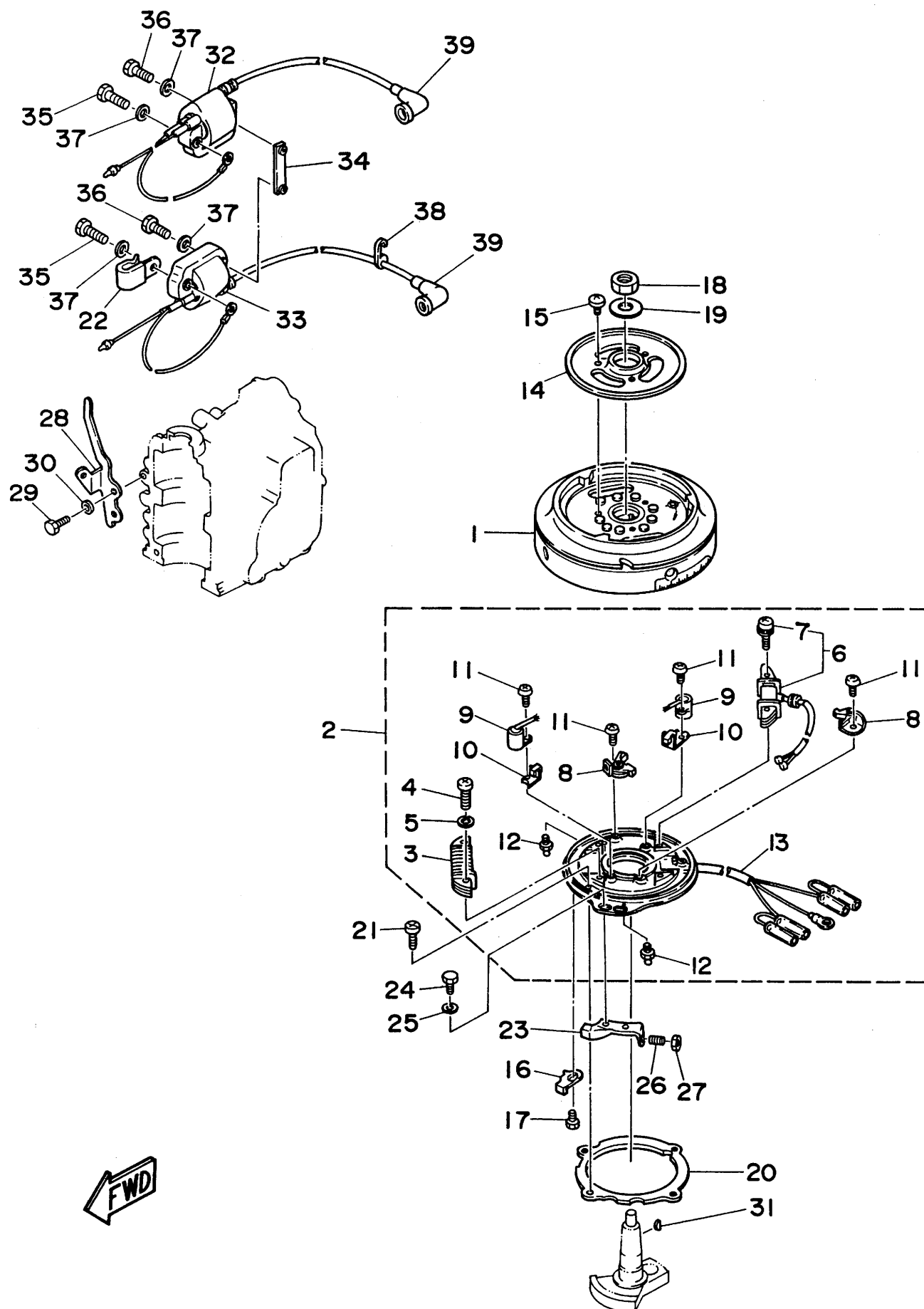
Fig. 13 ELECTRICAL 2 (POINT MODEL)
