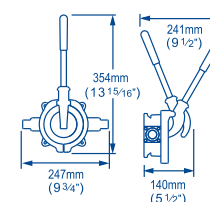
Bulkhead/Removable Handle BP9021 Plan View Side View
