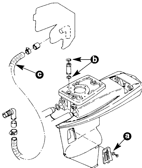
Figure 1. Raw Water Filter
