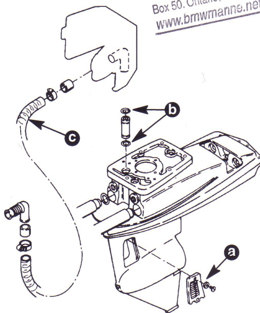
Figure 1. Raw Water Filter
