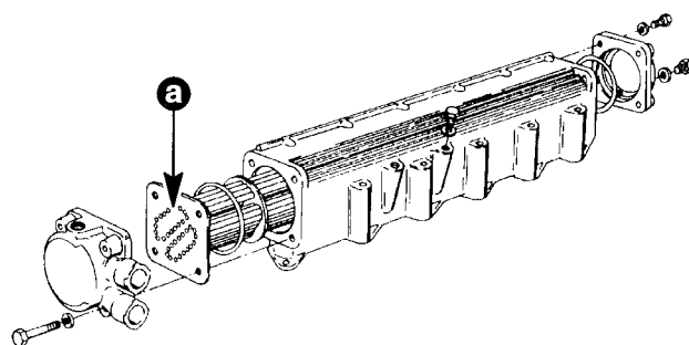
Figure 3. Sea Water Pump
